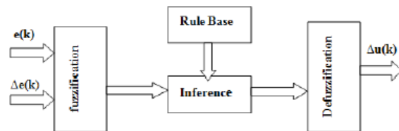
Fig 7. Fuzzy logic block diagram
