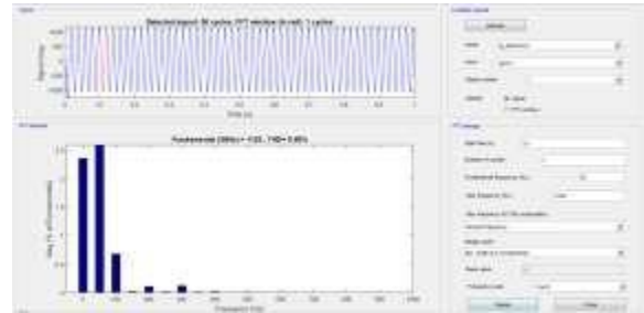
Fig 19. Extension system Current THD 0.69%
