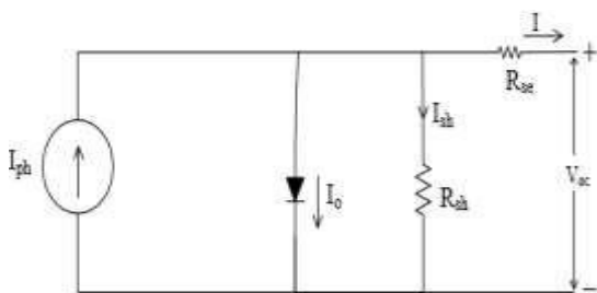
Fig. 2 Solar cell equivalent circuit
