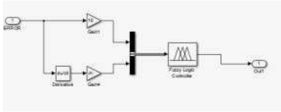
Fig 14.FUZZY controller subsystem
